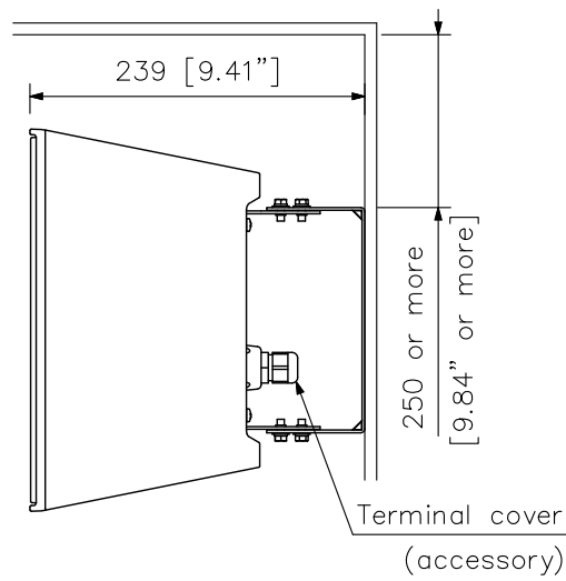
Vertical installation
